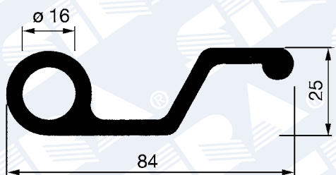
TENSIONER PROFILE
