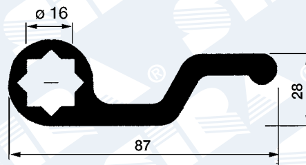
TENSIONER PROFILE
